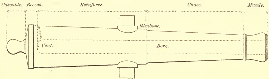
FIG. 8.—Field 6-pdr. smooth-bore Bronze Gun.
